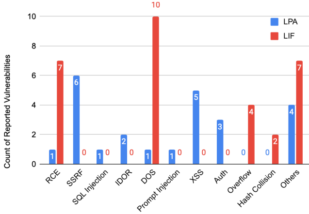
Figure 2: Comparison of Vulnerability Types.
